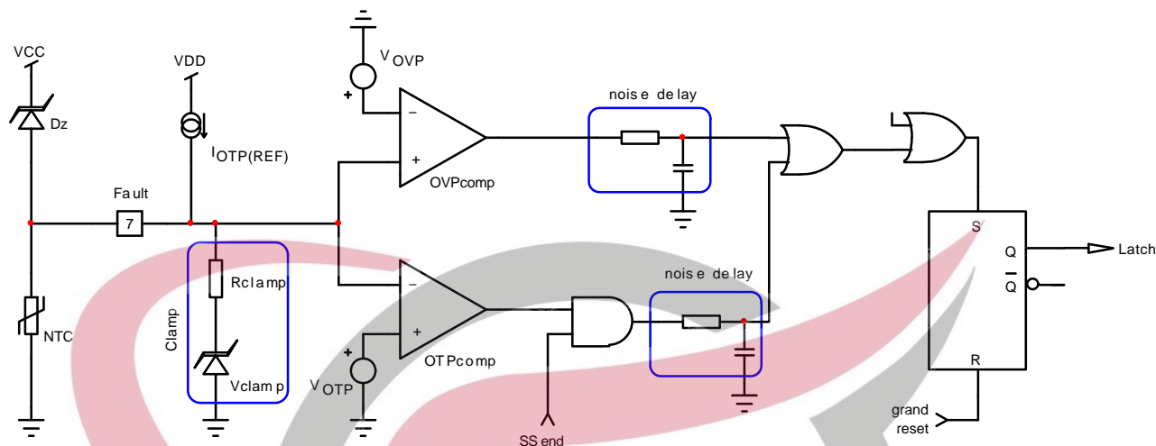
Figure 41. OVP/OTP Circuitry
